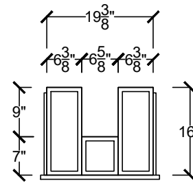
DRAWER BOX DETAIL
