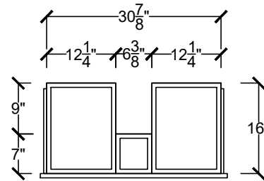
DRAWER BOX DETAIL
