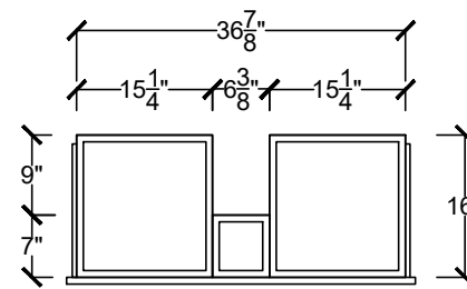
DRAWER BOX DETAIL
